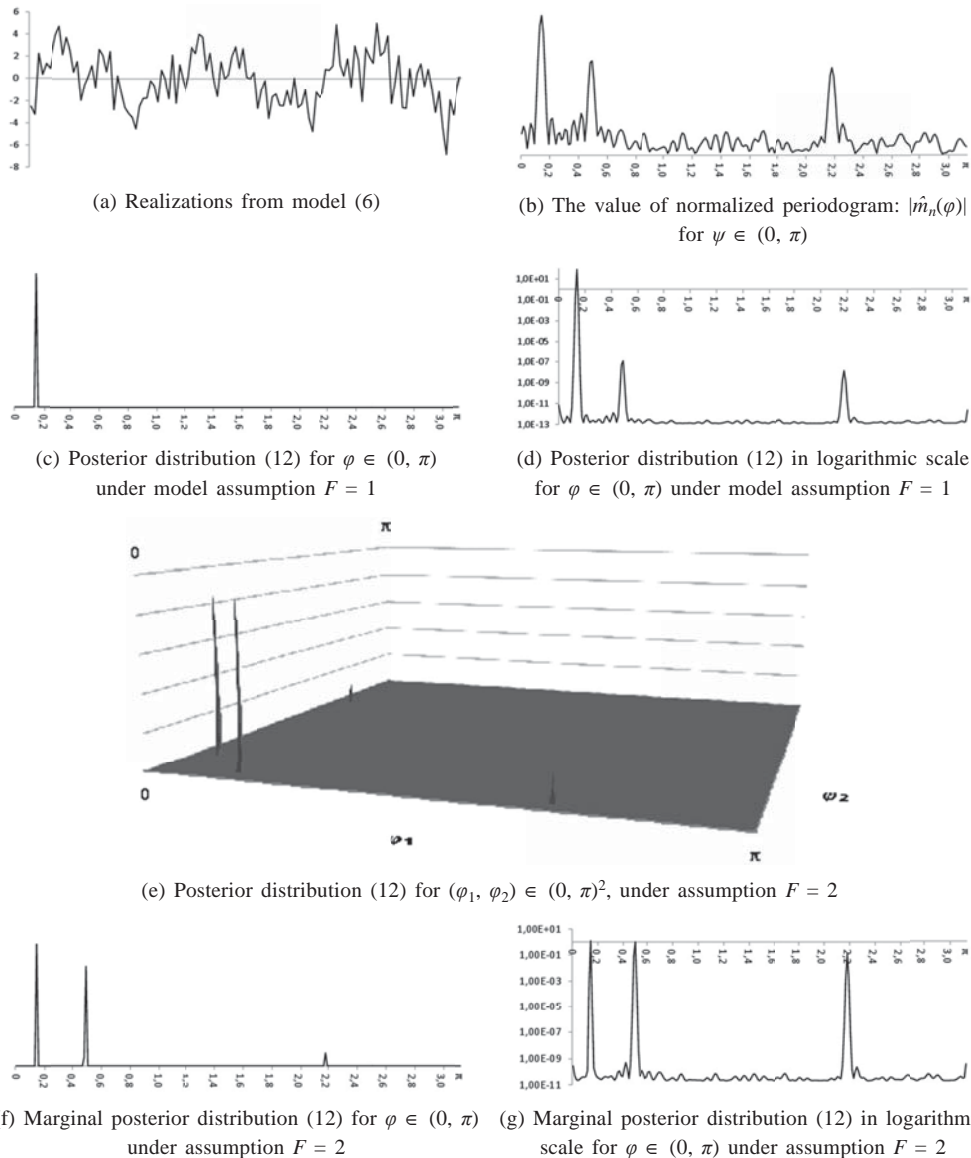
Figure 4. Posterior distributions in case of sample with length n = 120 generated from considered model (6) with F = 2 , \varphi_1 = 0.15 , \varphi_2 = 0.5 , \varphi_3 = 2.2 , a_1 = 2 , b_1 = 0 , a_2 = -1.5 , b_2 = 0 , a_3 = 0 , b_3 = 1.5 , \tau = 1
